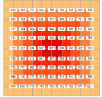
640W PPFD in 60cm
