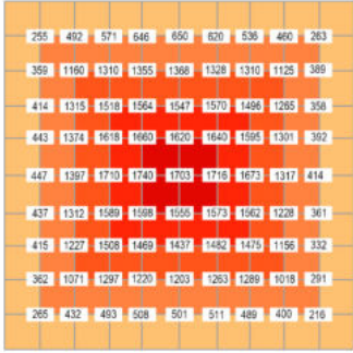
640W PPFD in 15cm
