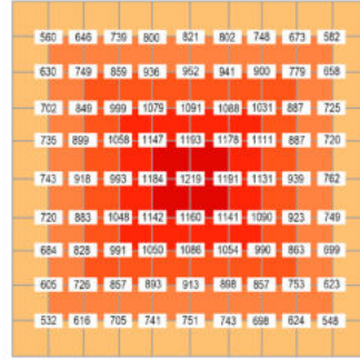
640W PPFD in 45cm
