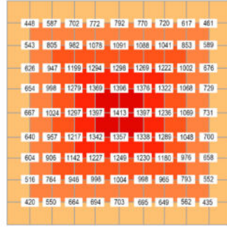
640W PPFD in 30cm
